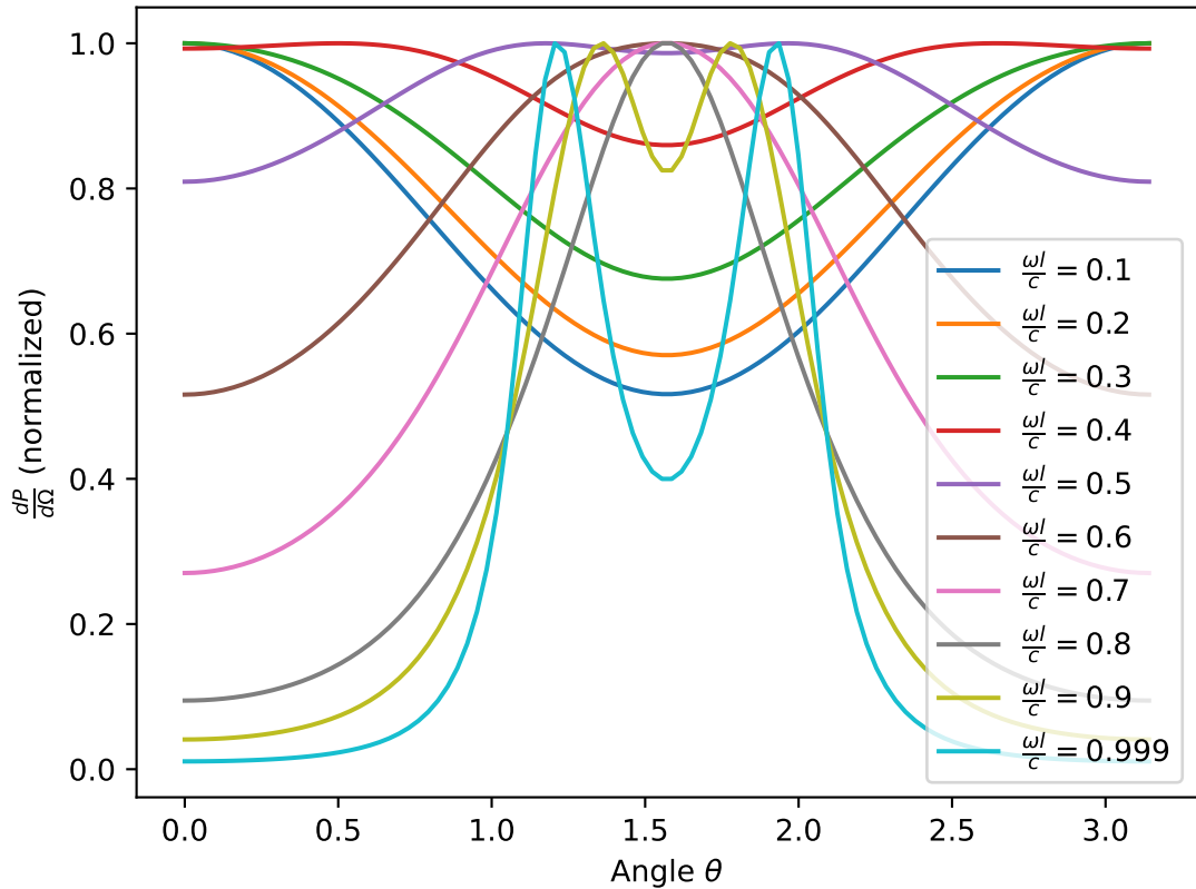
Angular Power Distribution as a Function of \frac{\omega l}{c}
