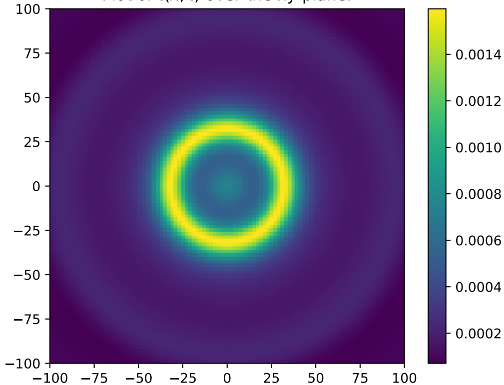
Plot of \tilde{t}(\vec{x}, t) over the xy-plane.
