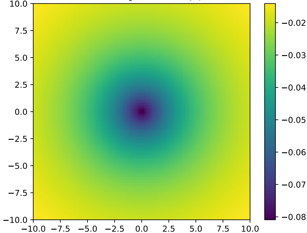
Plot of \tilde{t}(\vec{x}, t) + \frac{|\vec{x}|}{c} over the xy-plane.
