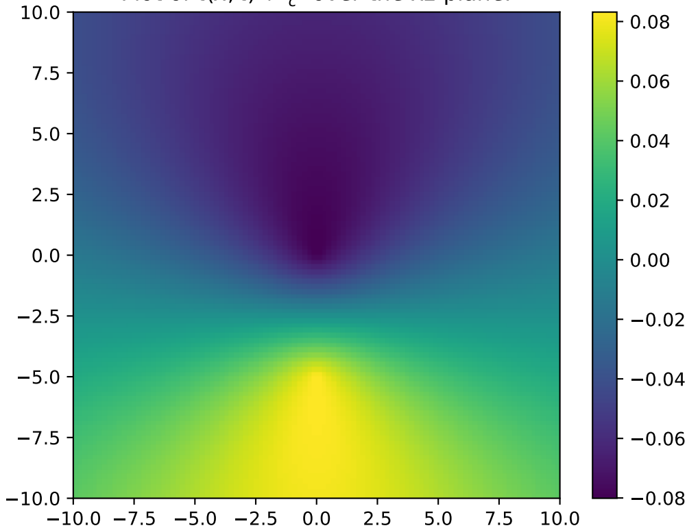
Plot of \tilde{t}(\vec{x}, t) + \frac{|\vec{x}|}{c} over the xz-plane.
