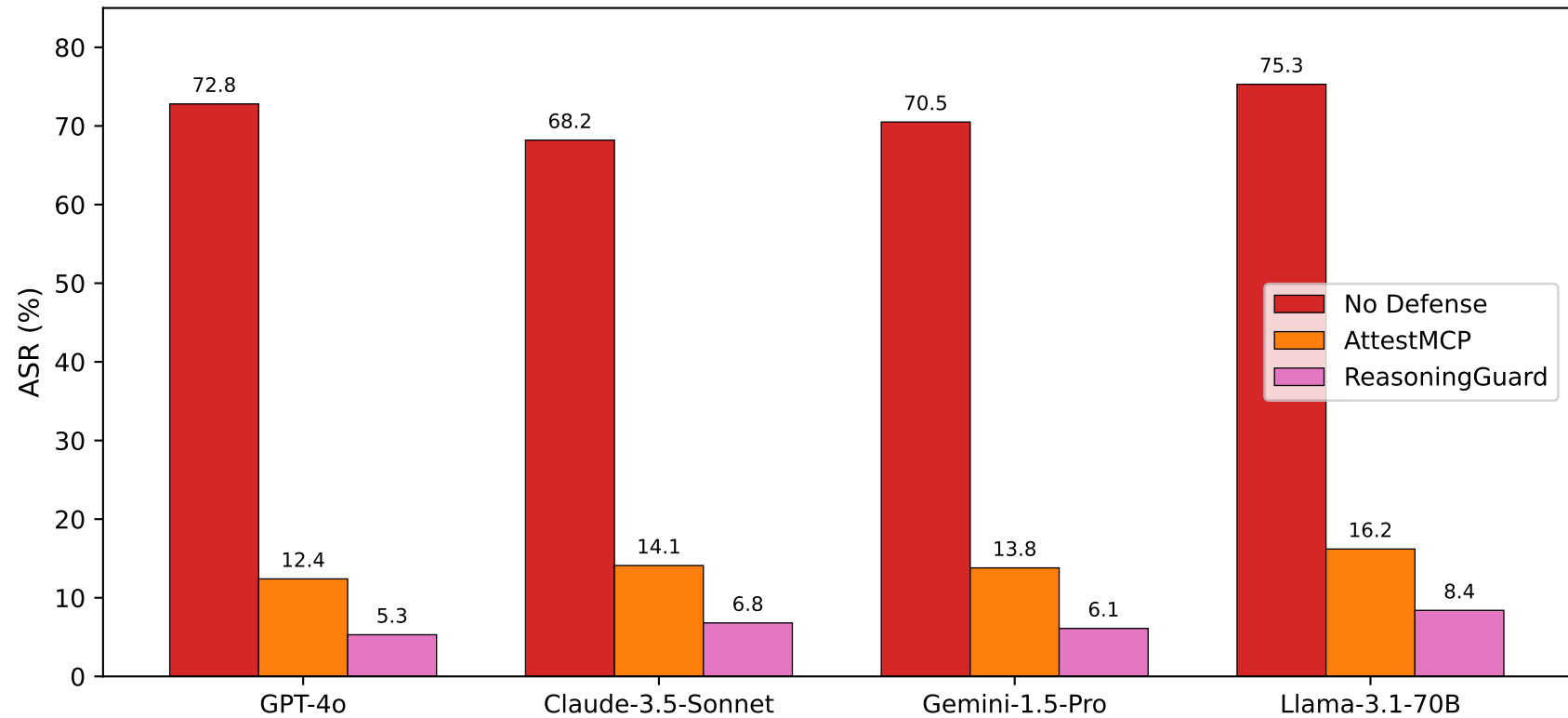
Multi-Model ASR Comparison
