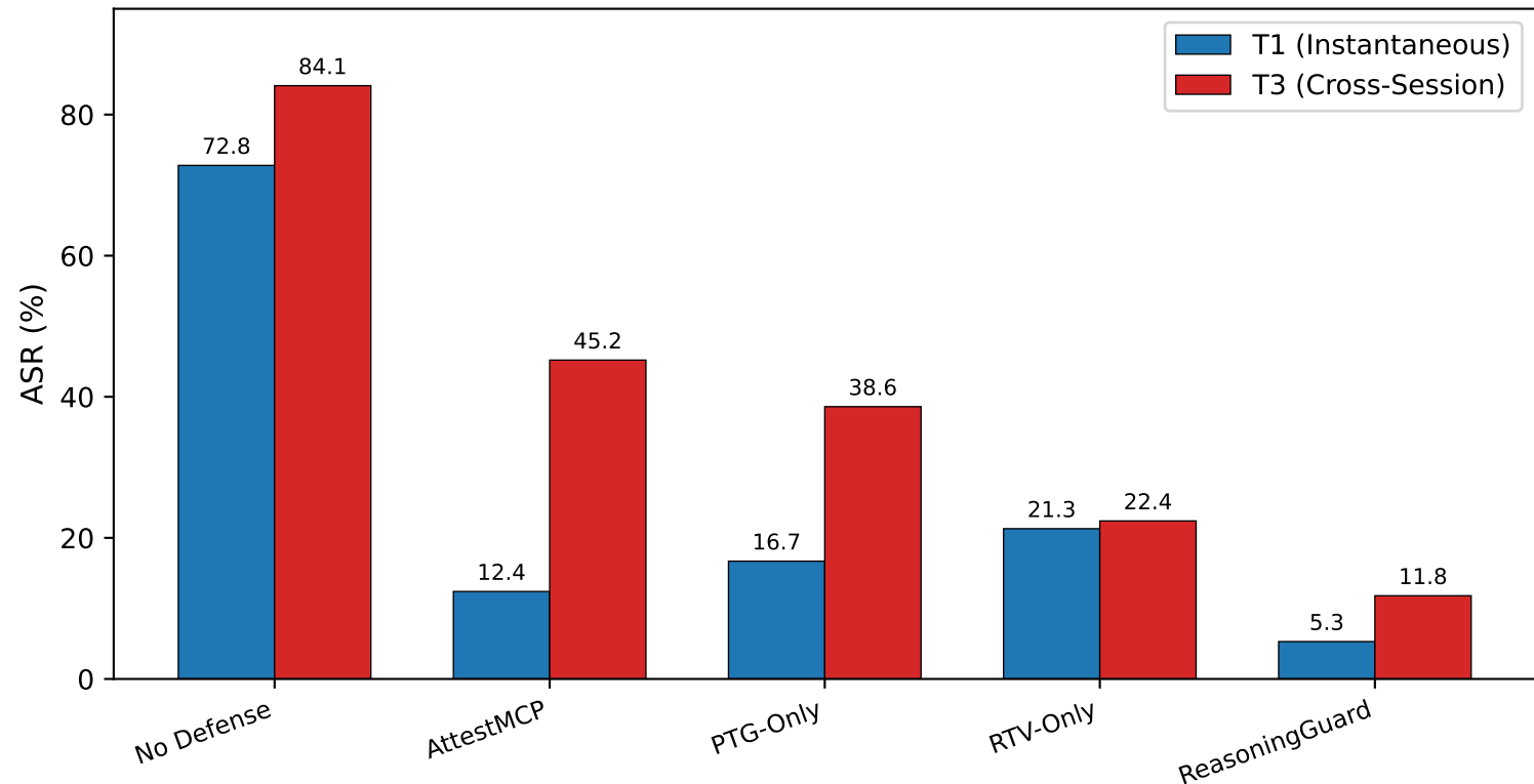
T1 vs T3 Attack Success Rate
