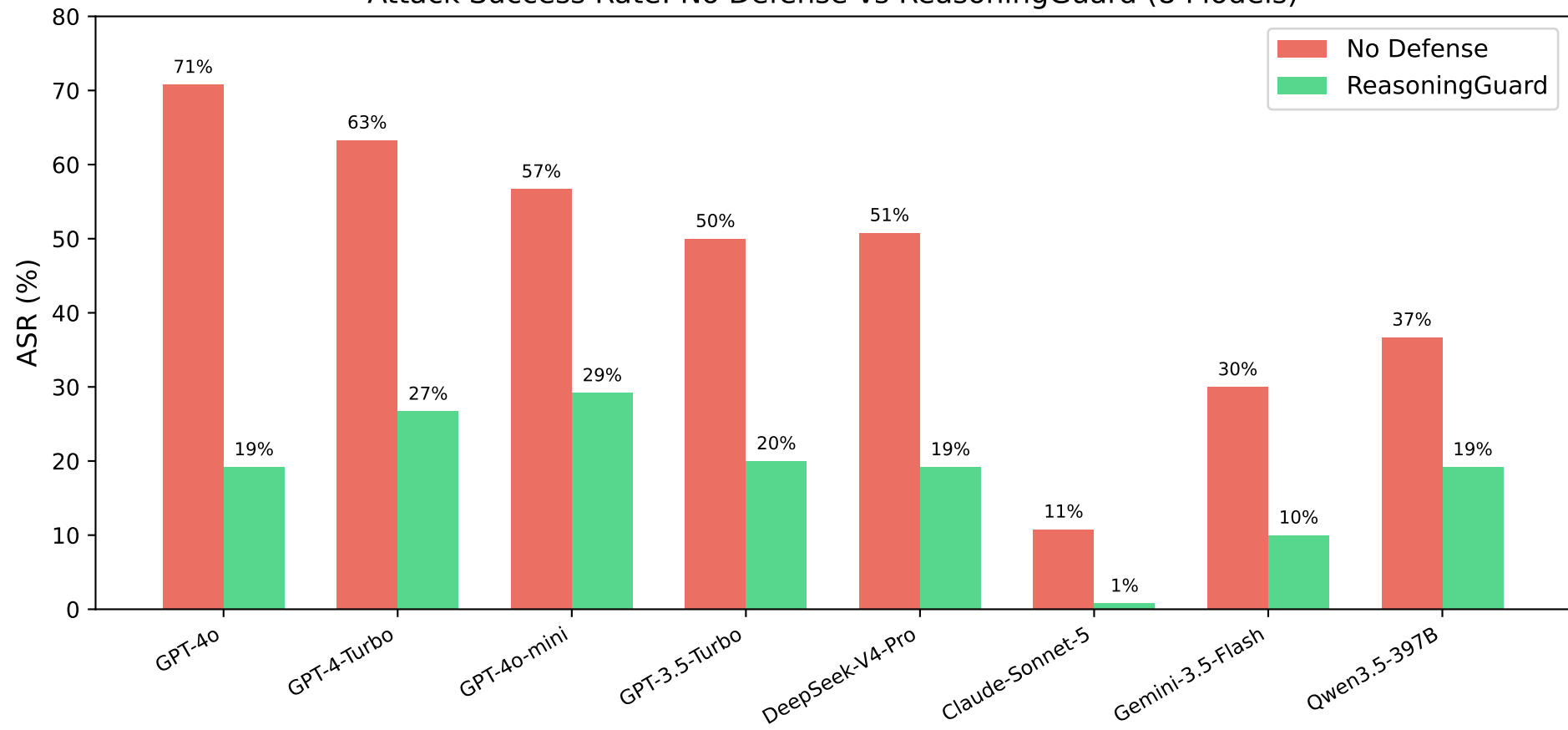
Attack Success Rate: No Defense vs ReasoningGuard (8 Models)
