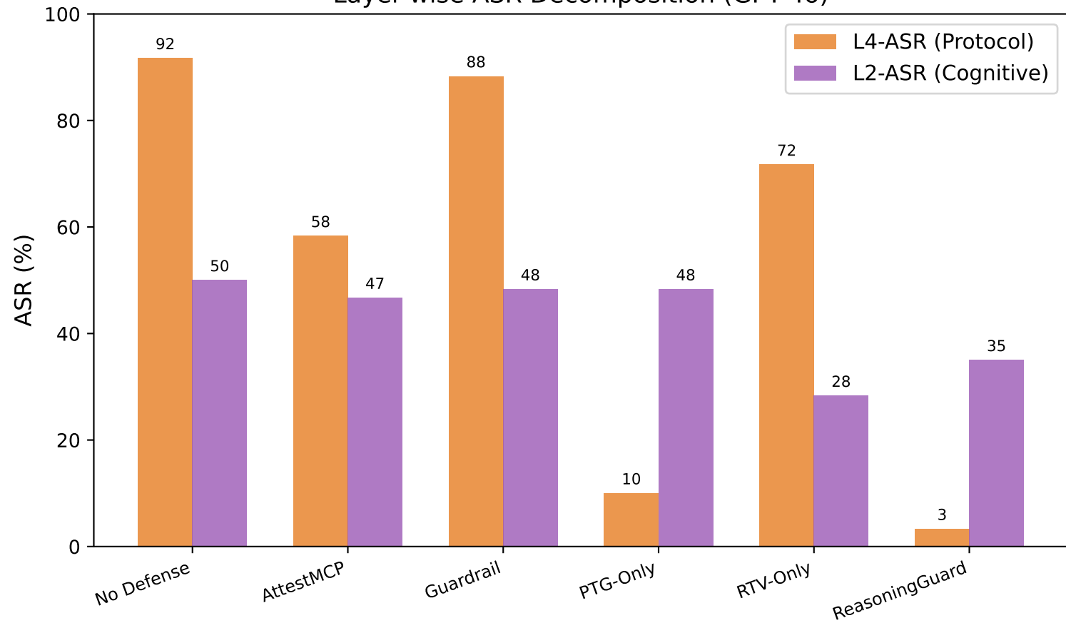
Layer-wise ASR Decomposition (GPT-4o)
