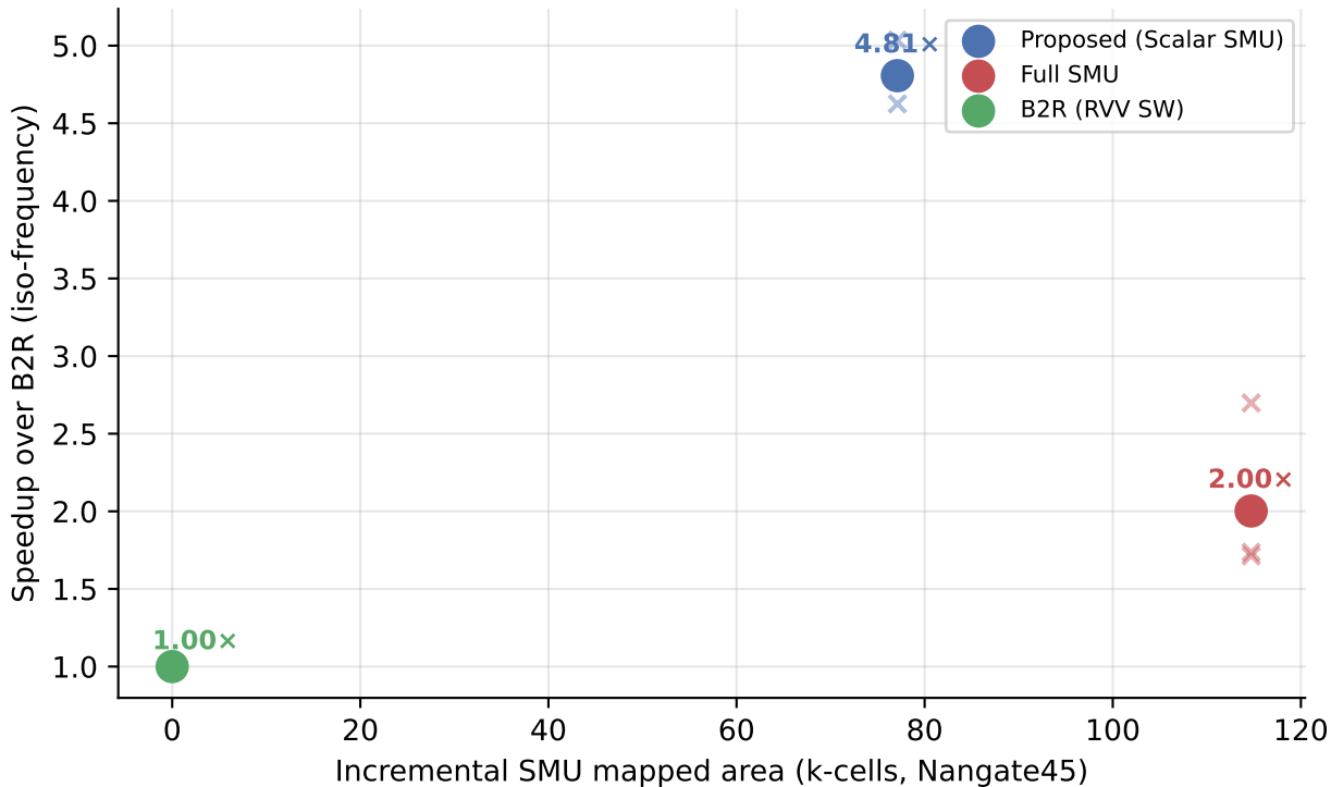
P12/P17 Figure 3 — performance-area trade-off (x=per workload: BERT / Mistral / Qwen14B; ●=geomean)
