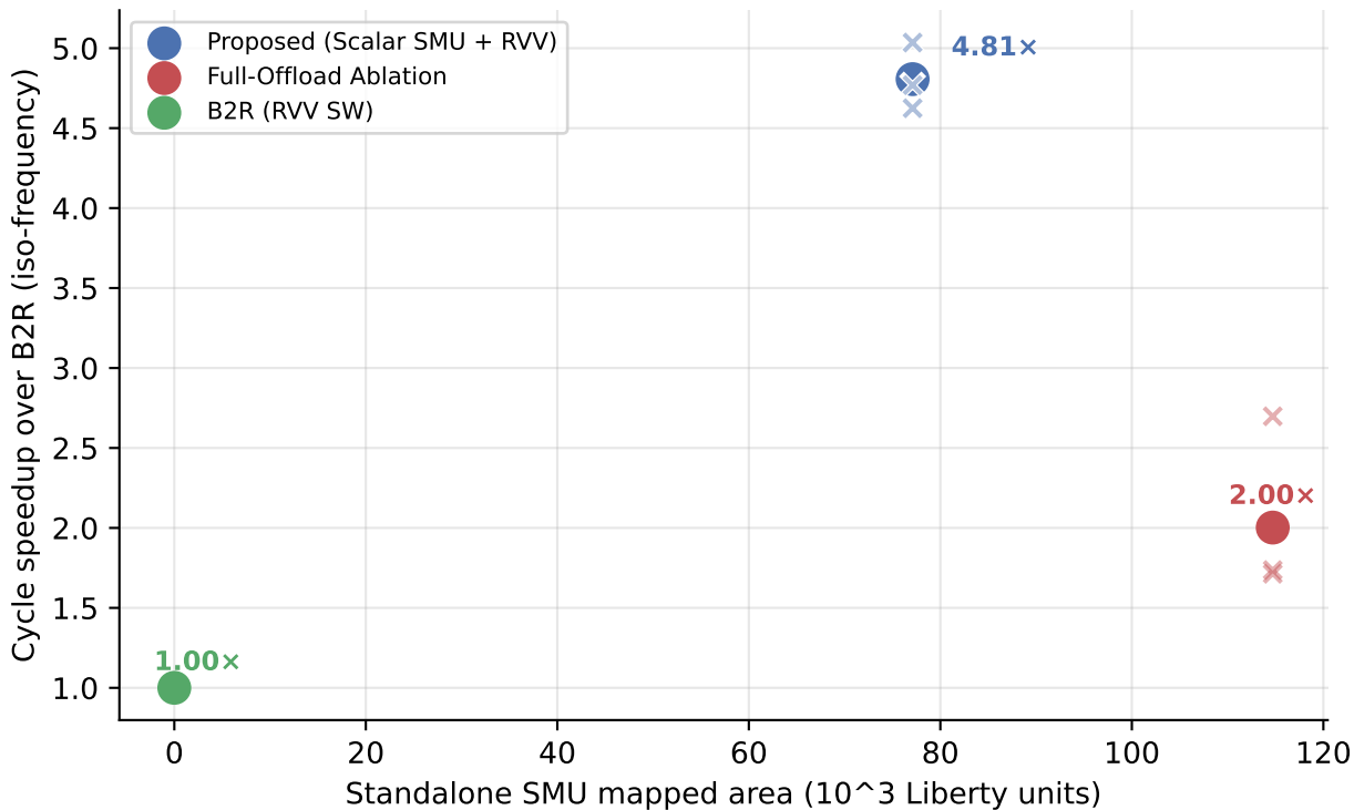
Performance-area trade-off (x=per workload: BERT / Mistral / Qwen14B; ●=geomean)
