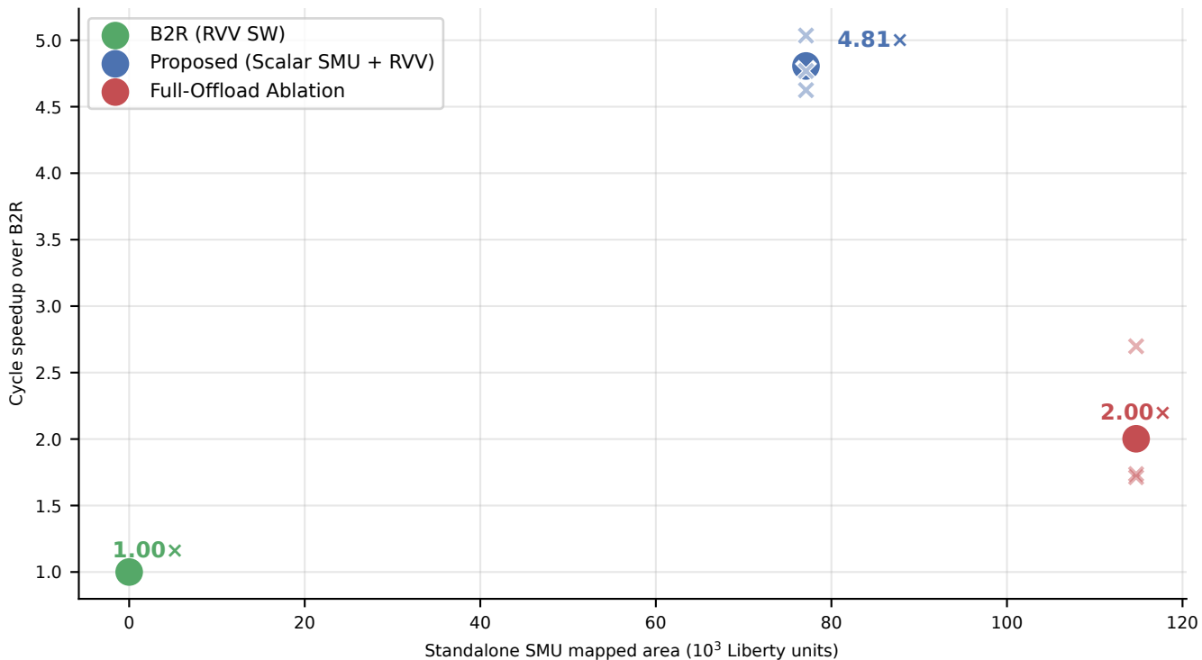
Performance-area trade-off ( \times =per workload: BERT / Mistral / Qwen14B; \bullet =geomean)
