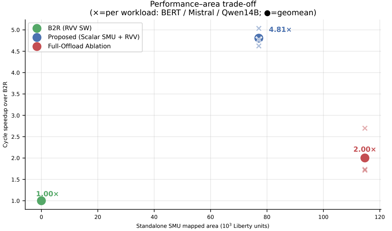
Fig. 3. Frequency-independent measured-cycle speedup over B2R versus standalone SMU mapped area. B2R’s zero SMU increment is not zero cluster area; circles mark geomeans and crosses mark workloads.
