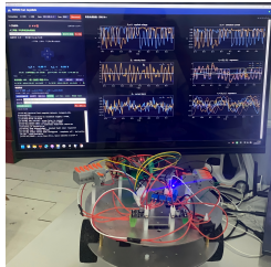
(a) Experimental platform
