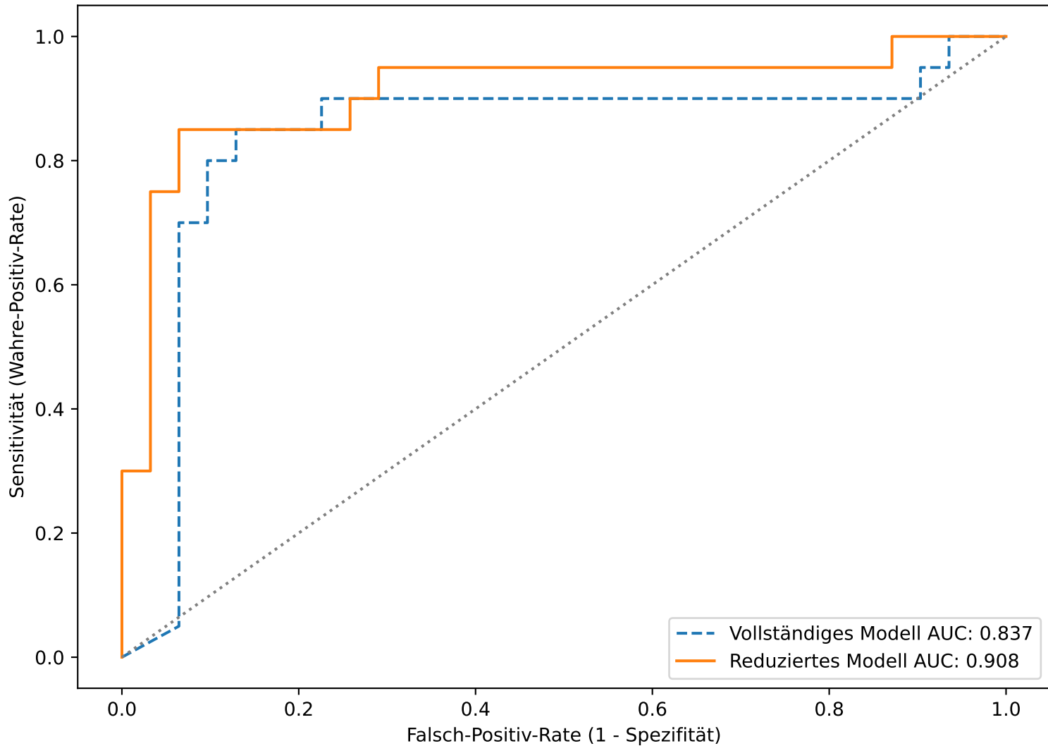
Cross-Validated ROC Curves
