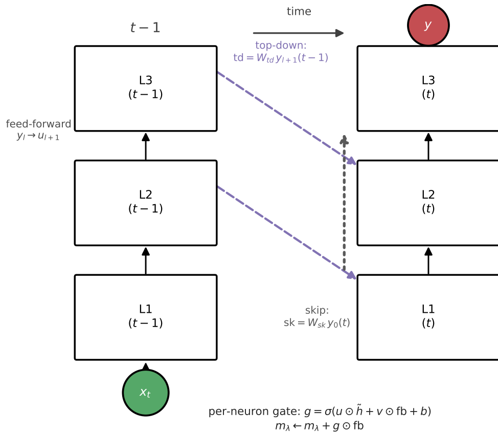
(a) Inter-layer feedback (top-down t - 1 + skip t )
