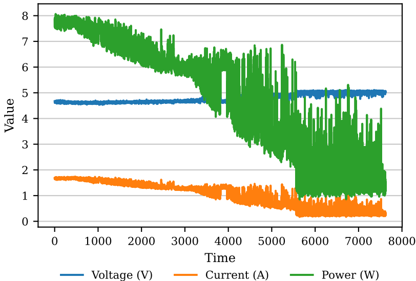
Voltage, Current, and Power Over Time
