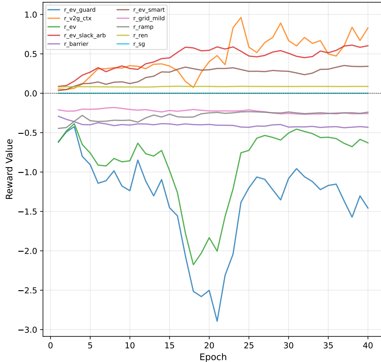
Grads Ablation (40ep)
