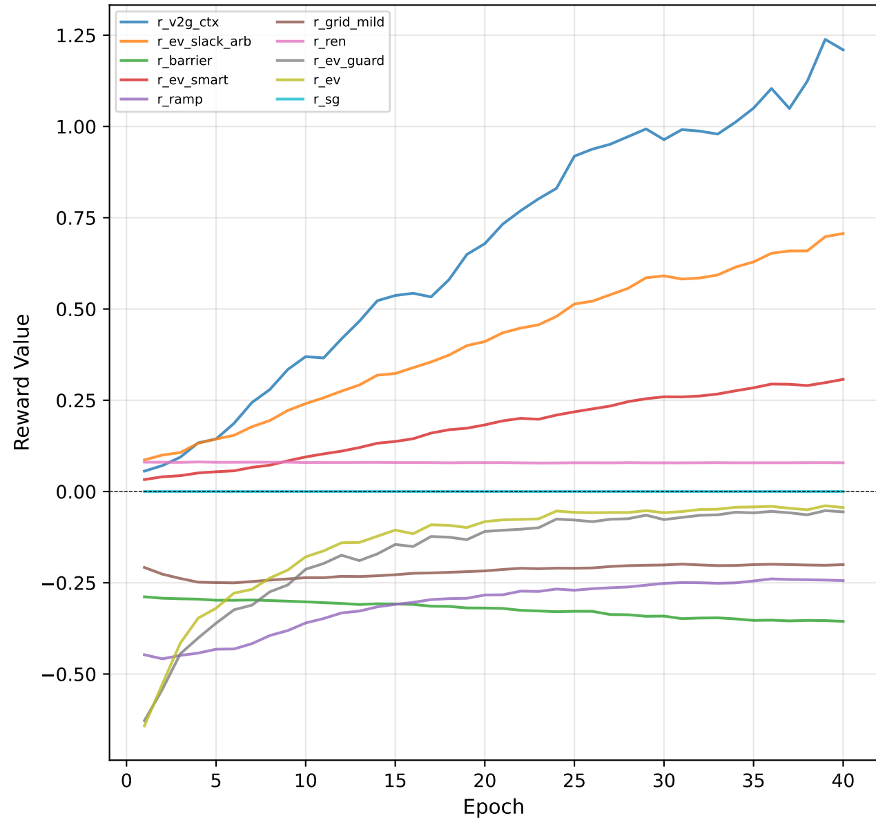
Softmax Ablation (40ep)
