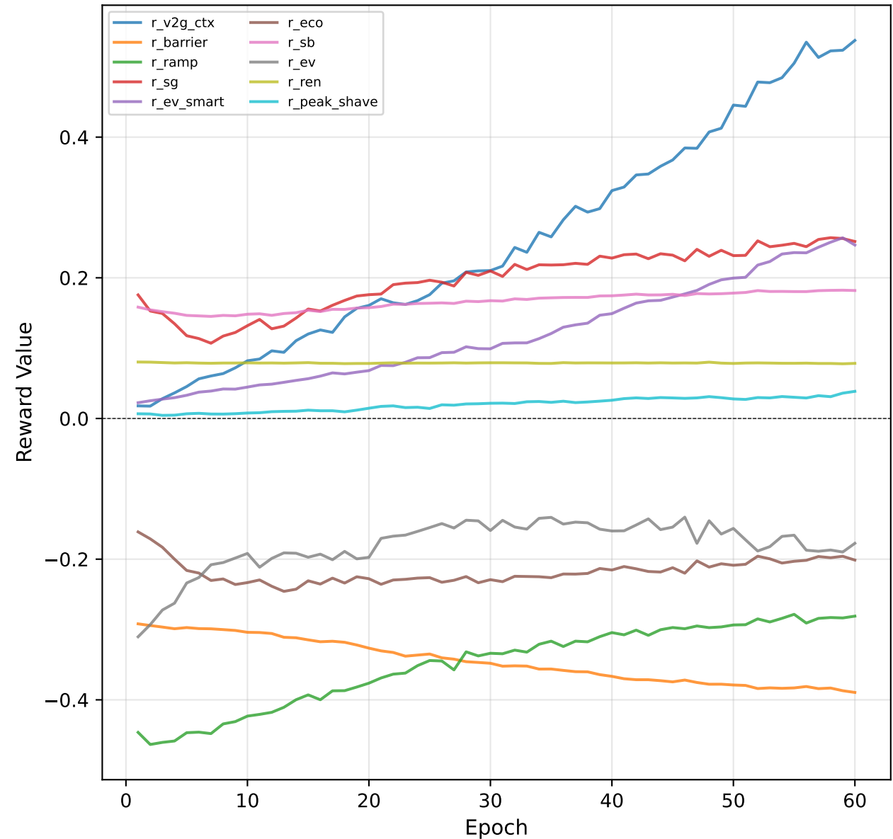
R28a Clean9 (60ep)
