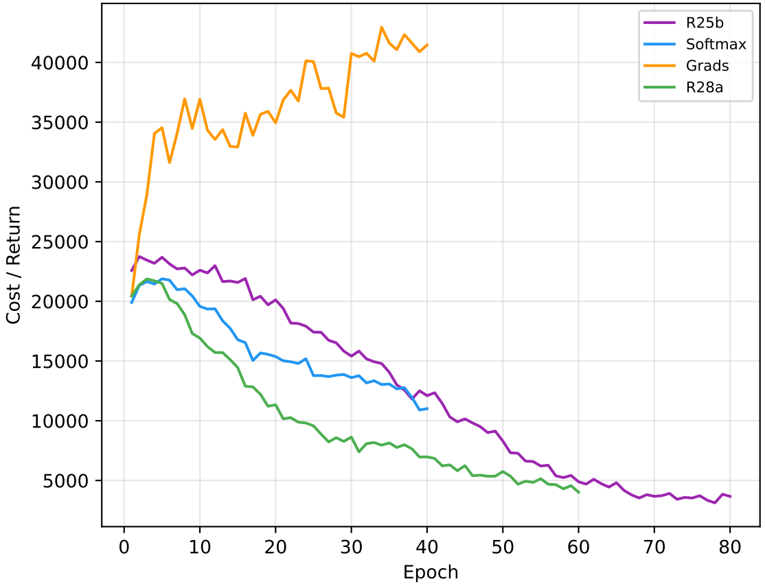
EpRet (Total Reward)
