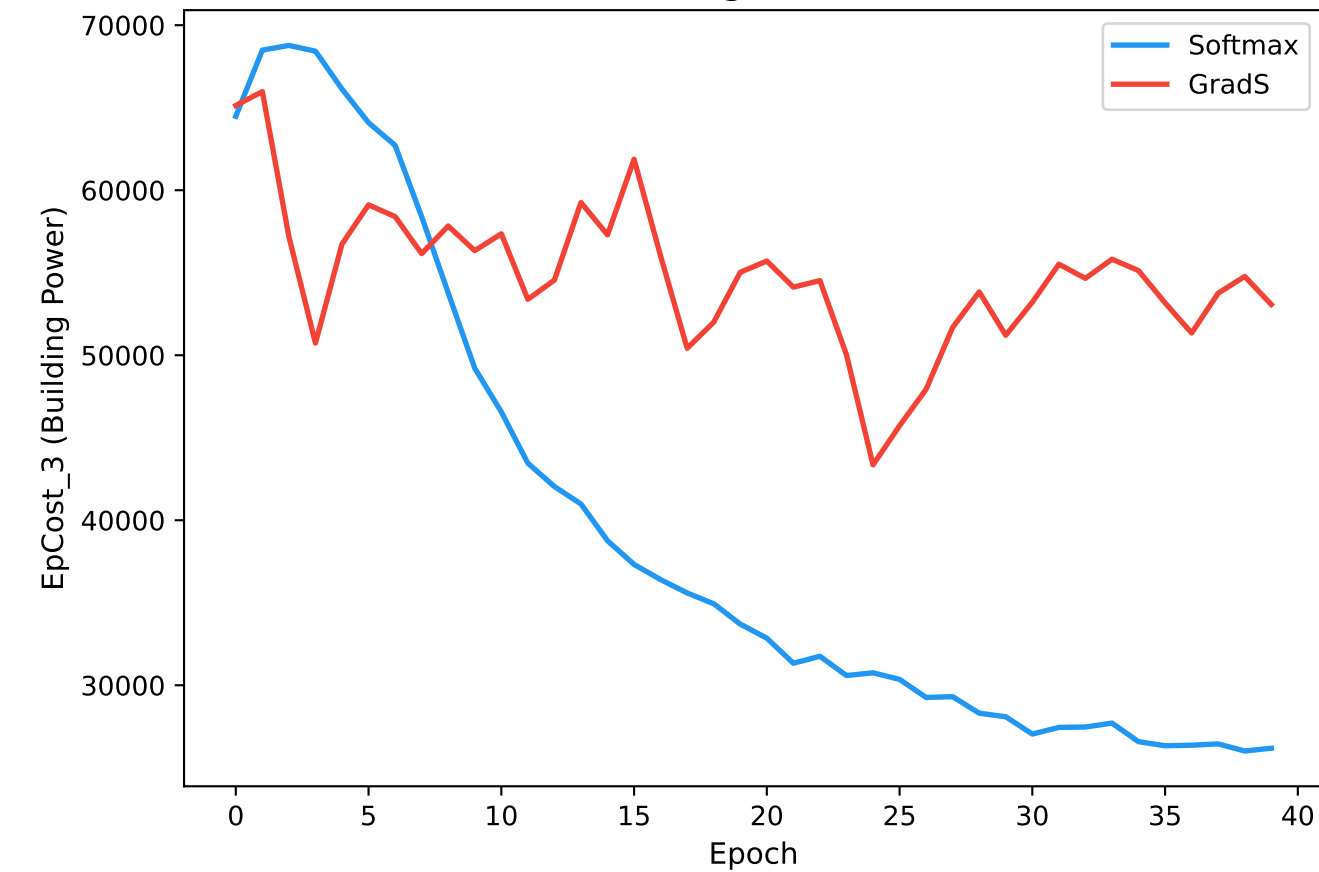
(c) C3: Building Power Violation
