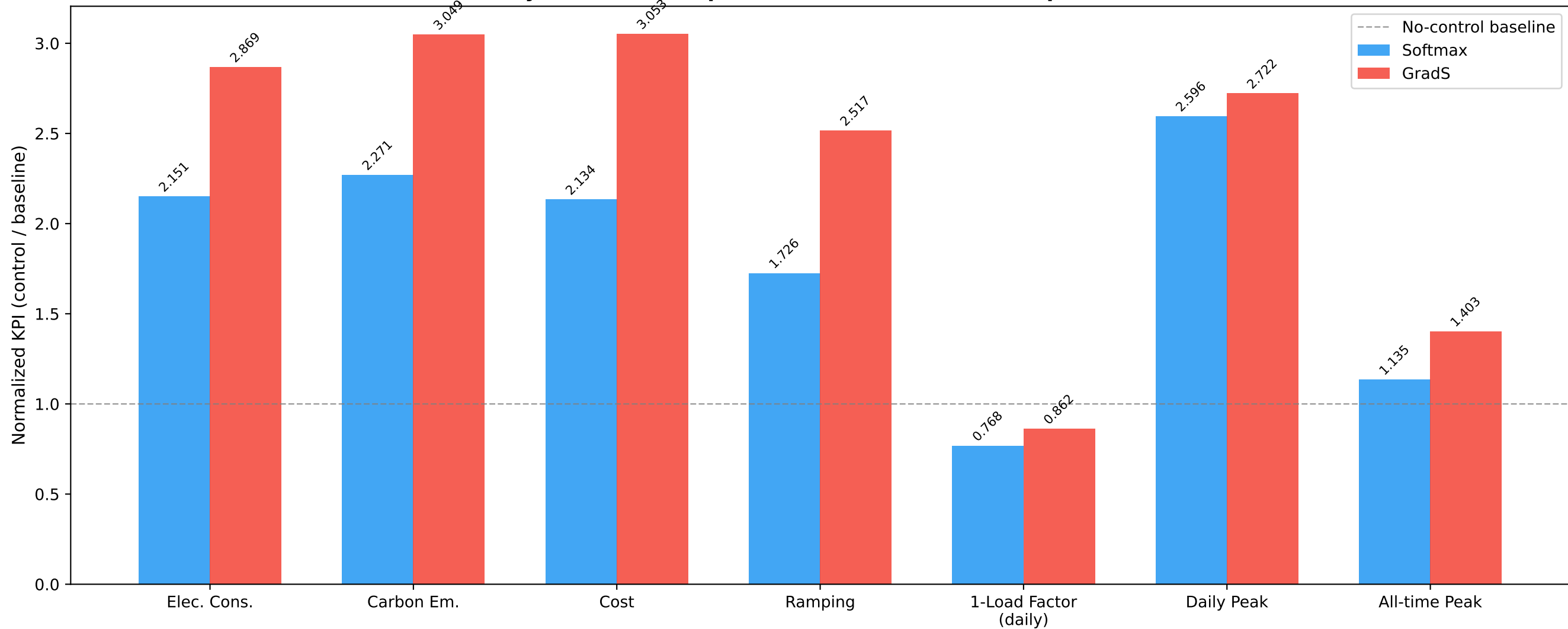
CityLearn KPI Comparison: Softmax vs GradS (Epoch 40)
