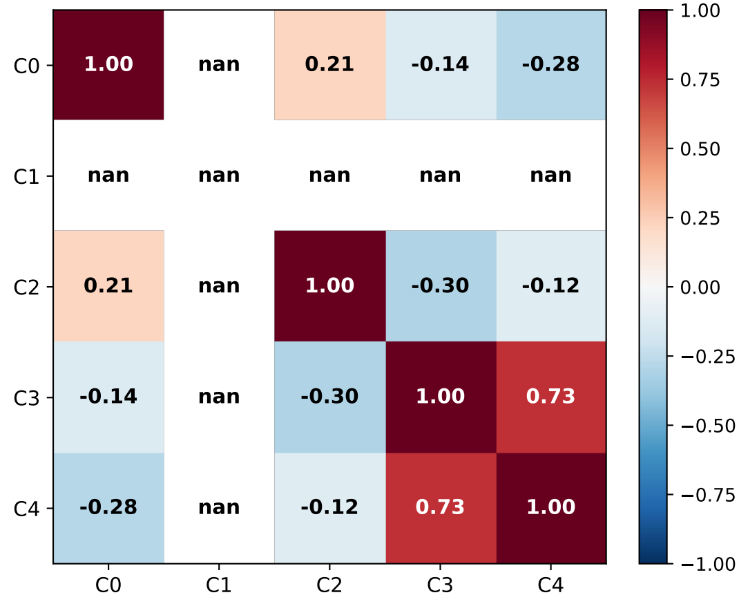
Pearson Correlation
