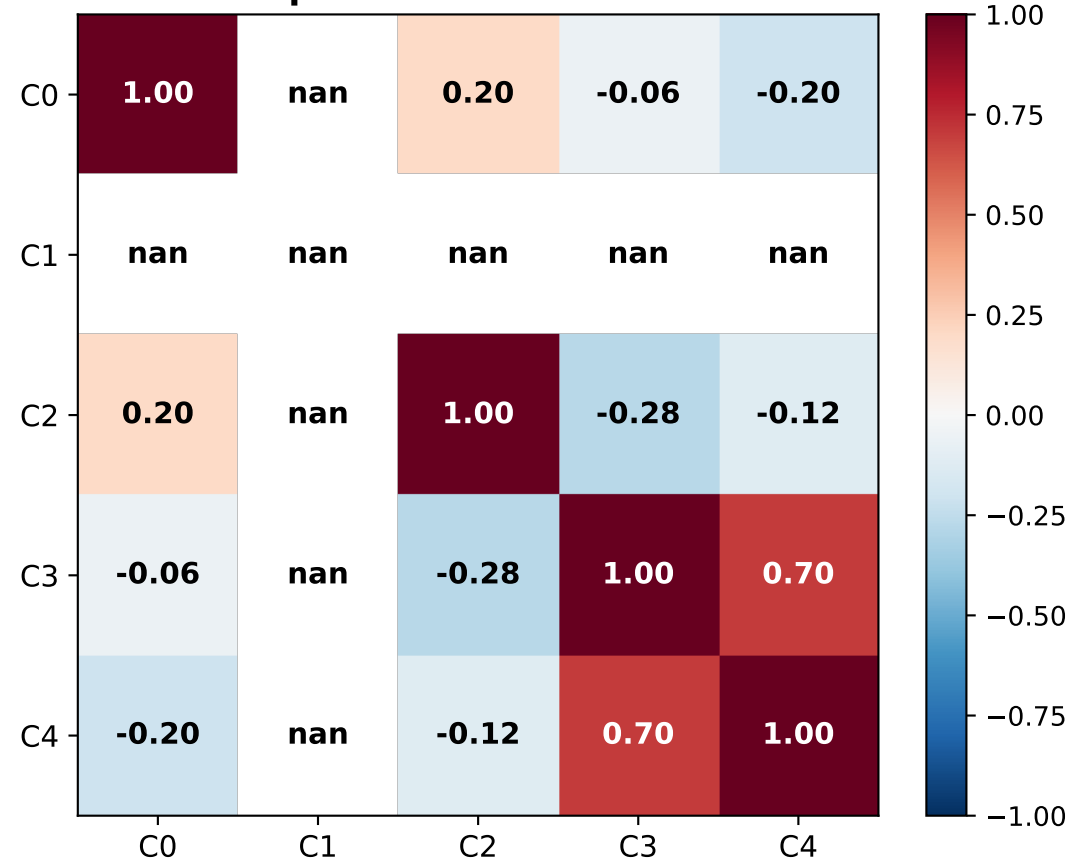
Spearman Correlation
