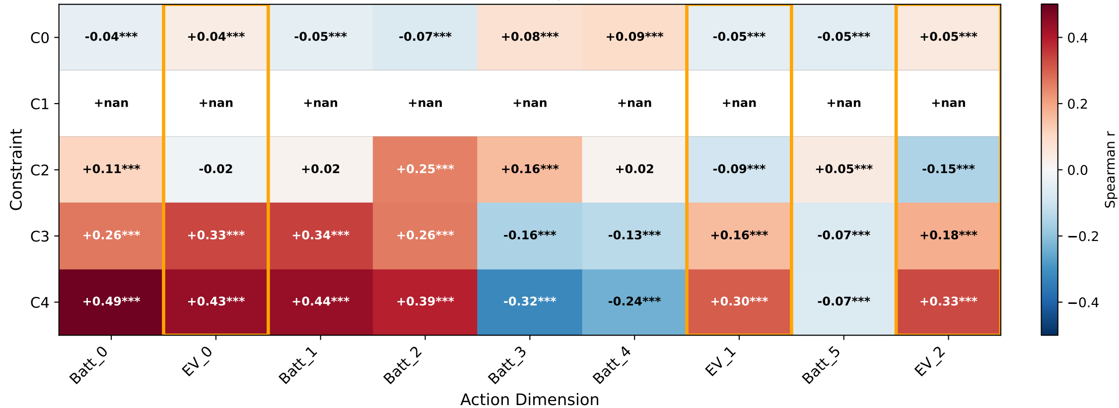
Action-Cost Sensitivity: Spearman Correlation (positive = action increases cost, negative = action decreases cost)
