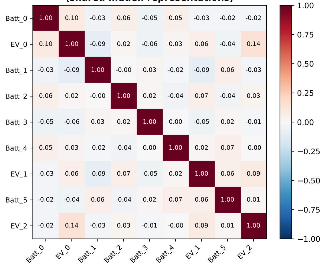
Action-Dim Weight Cosine Similarity (shared hidden representations)
