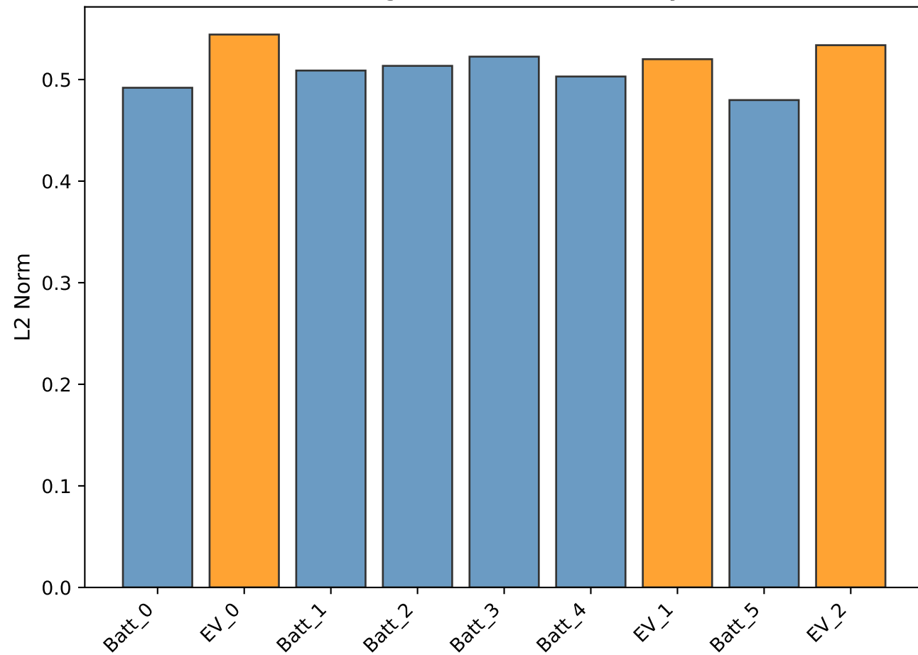
Last-Layer Weight Norms per Action (orange = EV, blue = Battery)
