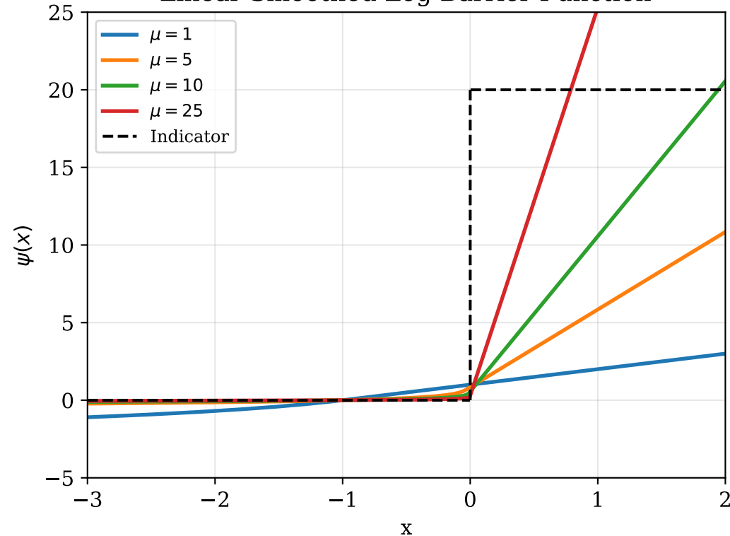
Linear Smoothed Log Barrier Function
