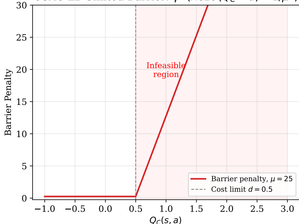
CSAC-LB Shifted Barrier: \psi^*(\text{ReLU}(Q_C - d) - 1/\mu^2)
