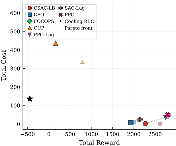
Reward--Cost Trade-off
