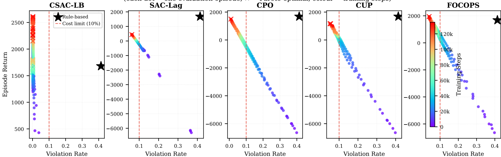
Evaluation Trajectory during Training (each dot = one evaluation episode, × = Pareto-optimal, colour = training steps)
