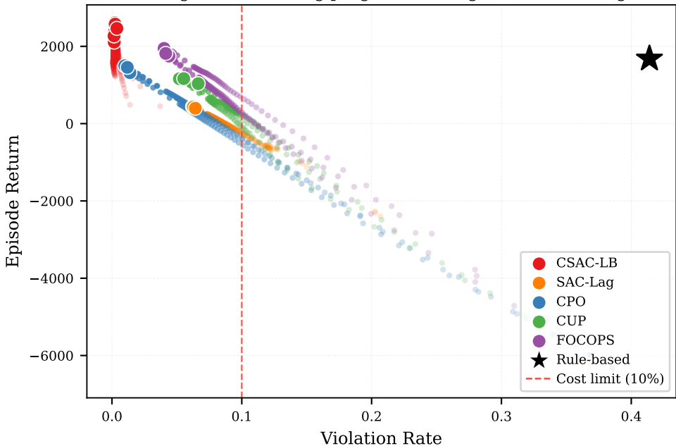
Evaluation Trajectory during Training — All Algorithms (fading dots = training progression; bright = late training)
