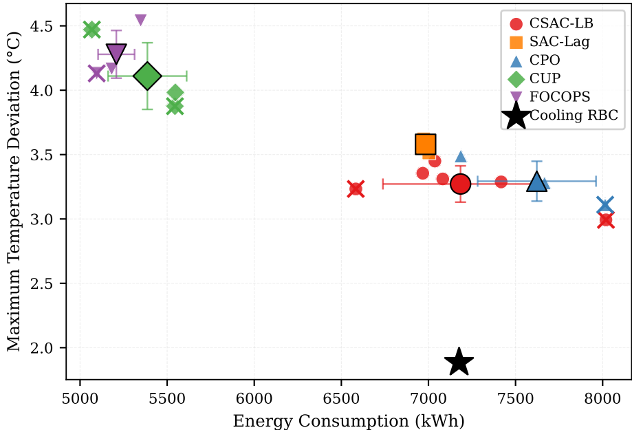
Energy Consumption vs. Maximum Temperature Deviation ( \times = Pareto-optimal seeds; large markers = mean \pm std over seeds)
