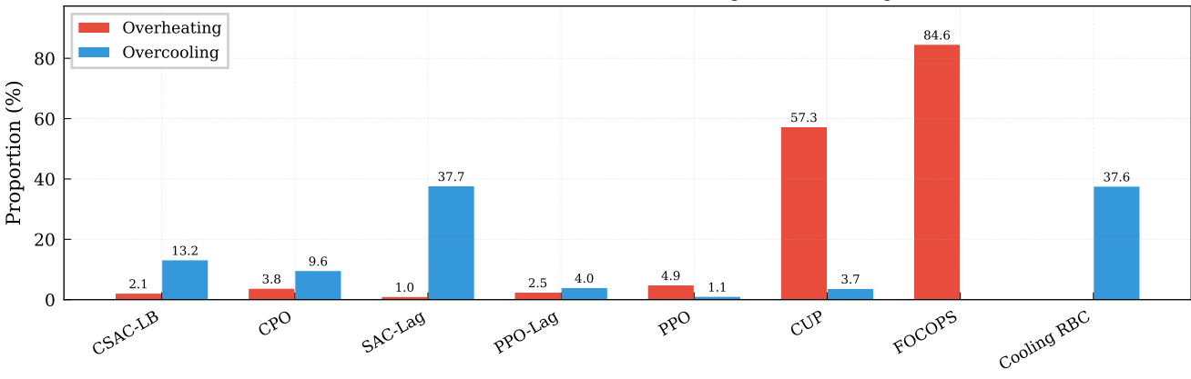
Discomfort Breakdown — Overheating vs Overcooling
