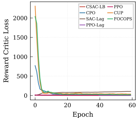
(b) Reward Critic Loss
