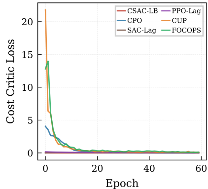
(c) Cost Critic Loss
