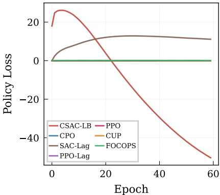
(a) Policy Loss
