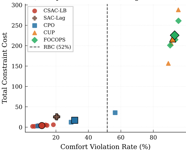
Constraint Cost vs. Violation Rate (each point = one seed; large = mean)
