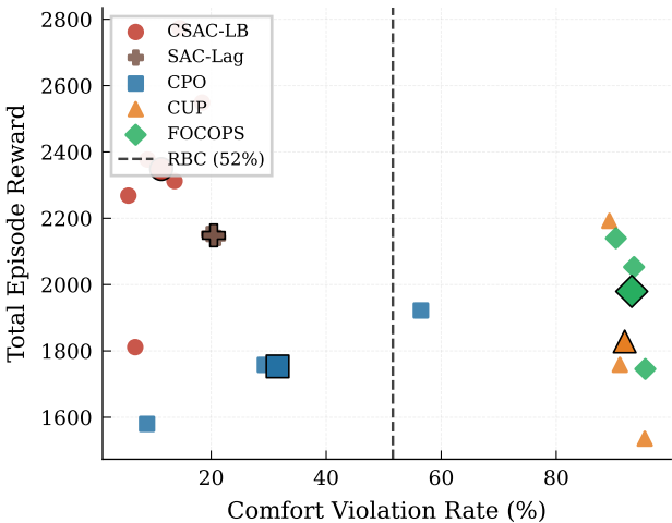
Reward vs. Violation Rate (each point = one seed; large = mean)
