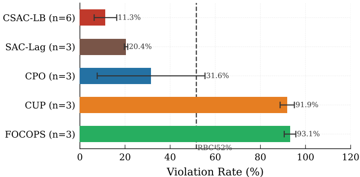
(a) Safety: Violation Rate
