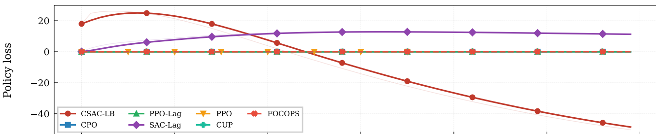
(e) Policy loss
