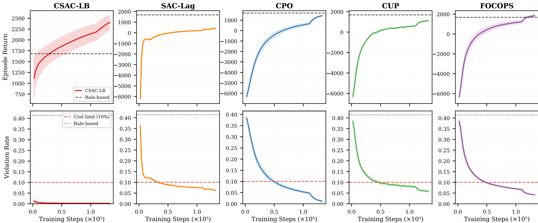
Training Dynamics: Mean \pm Std over Seeds (top: episode return; bottom: violation rate; dashed red = cost limit)
