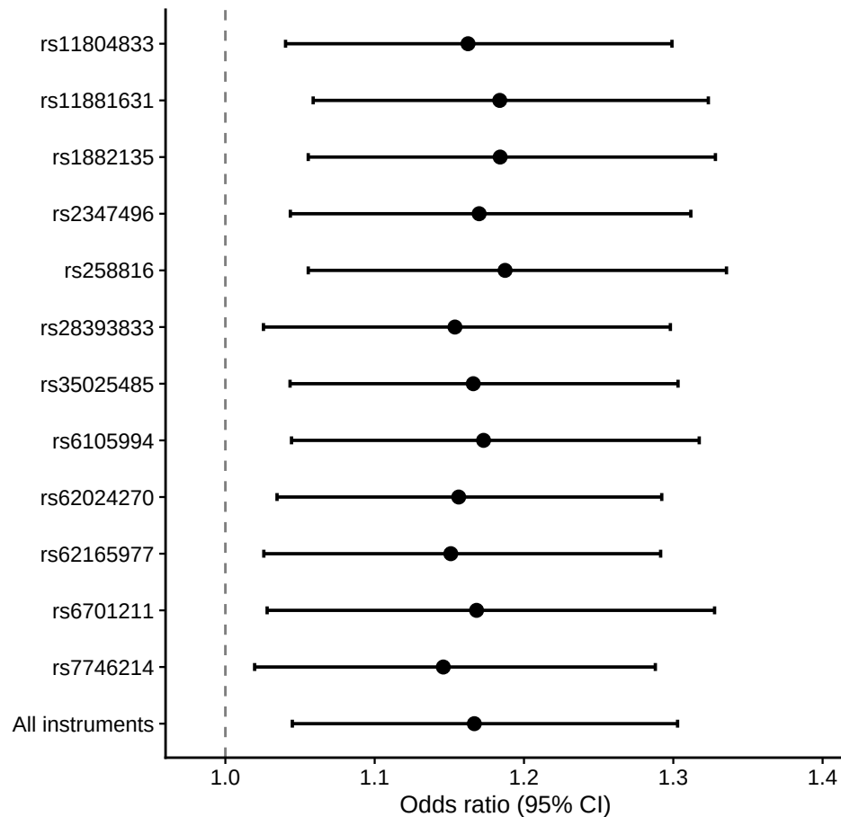
b Leave-one-out estimates
