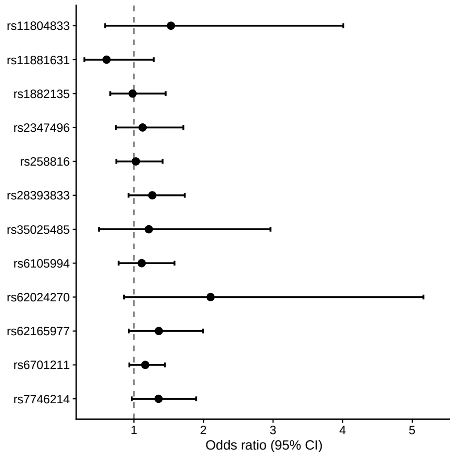
a Single-SNP estimates
