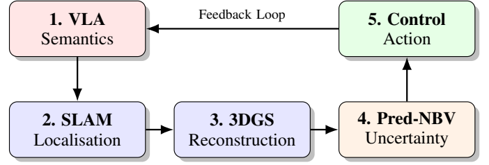
Fig. 1. The proposed Semantic-Metric Loop. A closed-loop architecture integrating VLA cognitive reasoning, 3DGS metric reconstruction, and Pred-NBV active exploration for edge-deployed autonomous UAVs.
