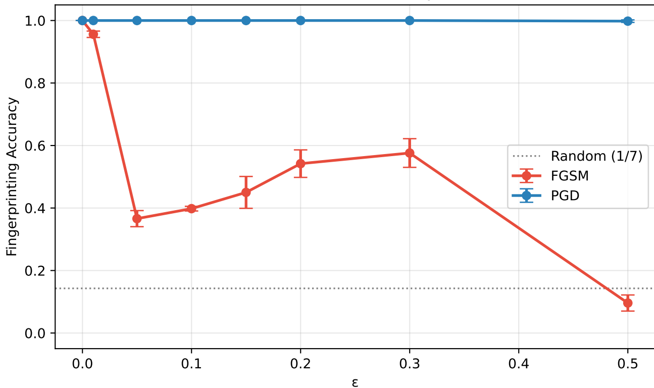
SARP IQ2CH — Accuracy vs \epsilon
