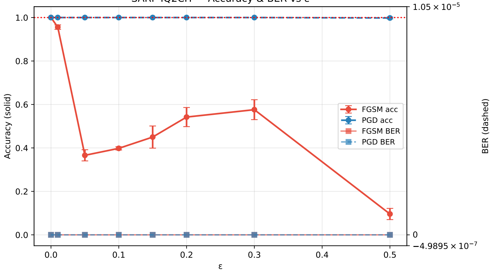
SARP IQ2CH — Accuracy & BER vs \epsilon
