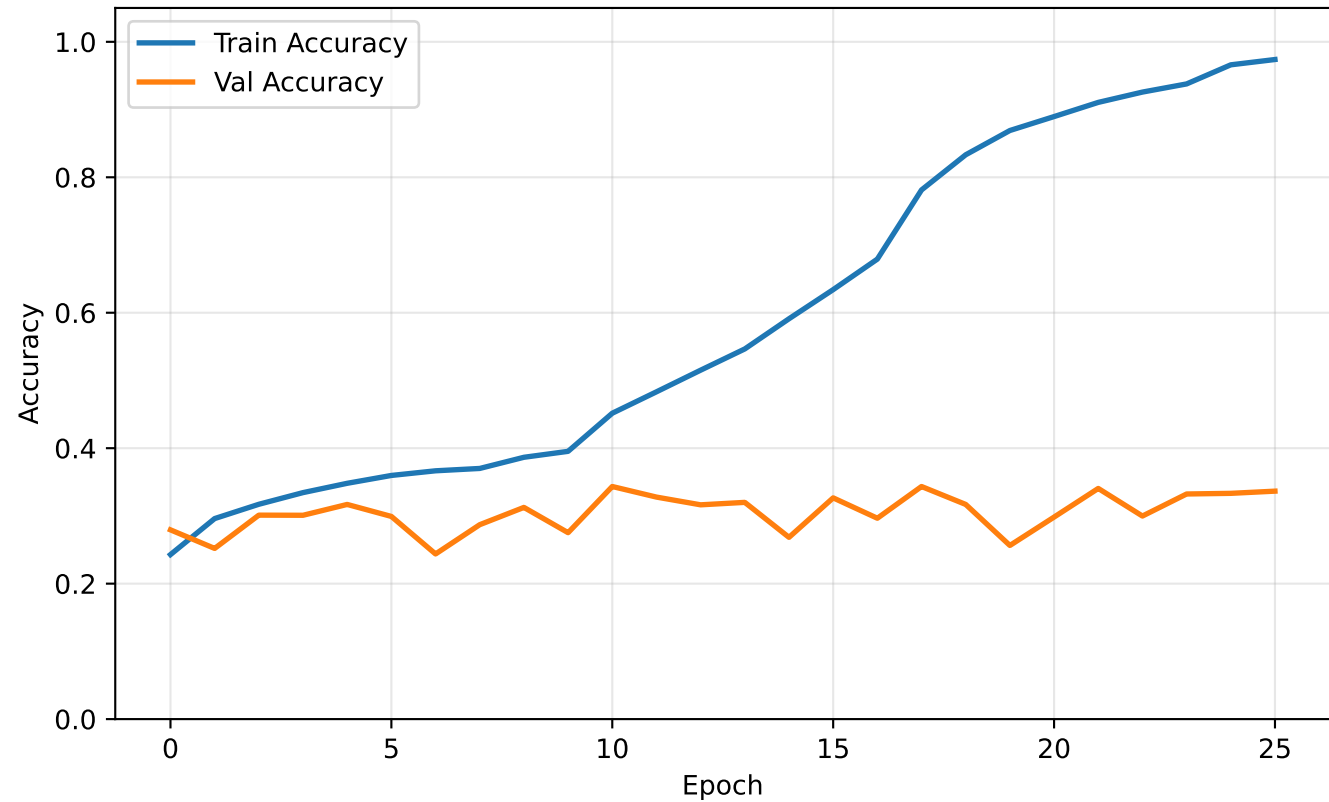
Training & Validation Accuracy
