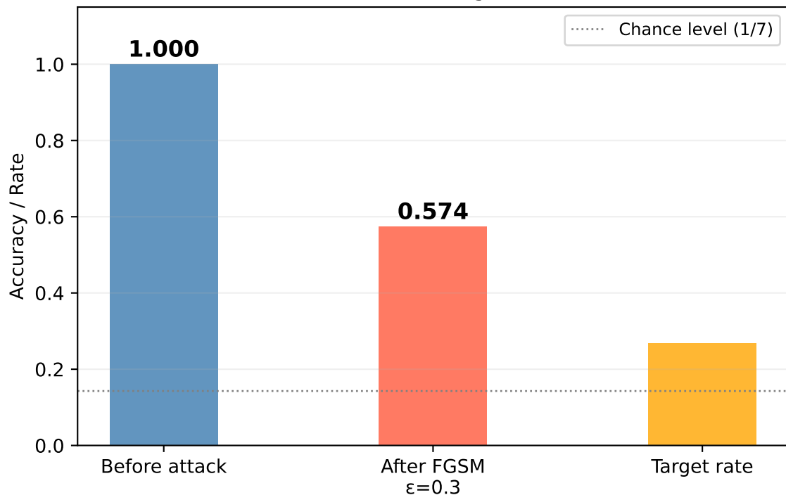
FGSM — Class 4 [Targeted→Dev2]
