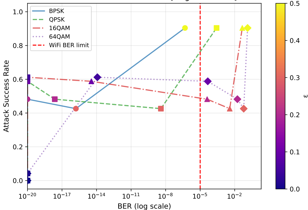
FGSM — Stealthiness Tradeoff [Targeted→Dev2]
