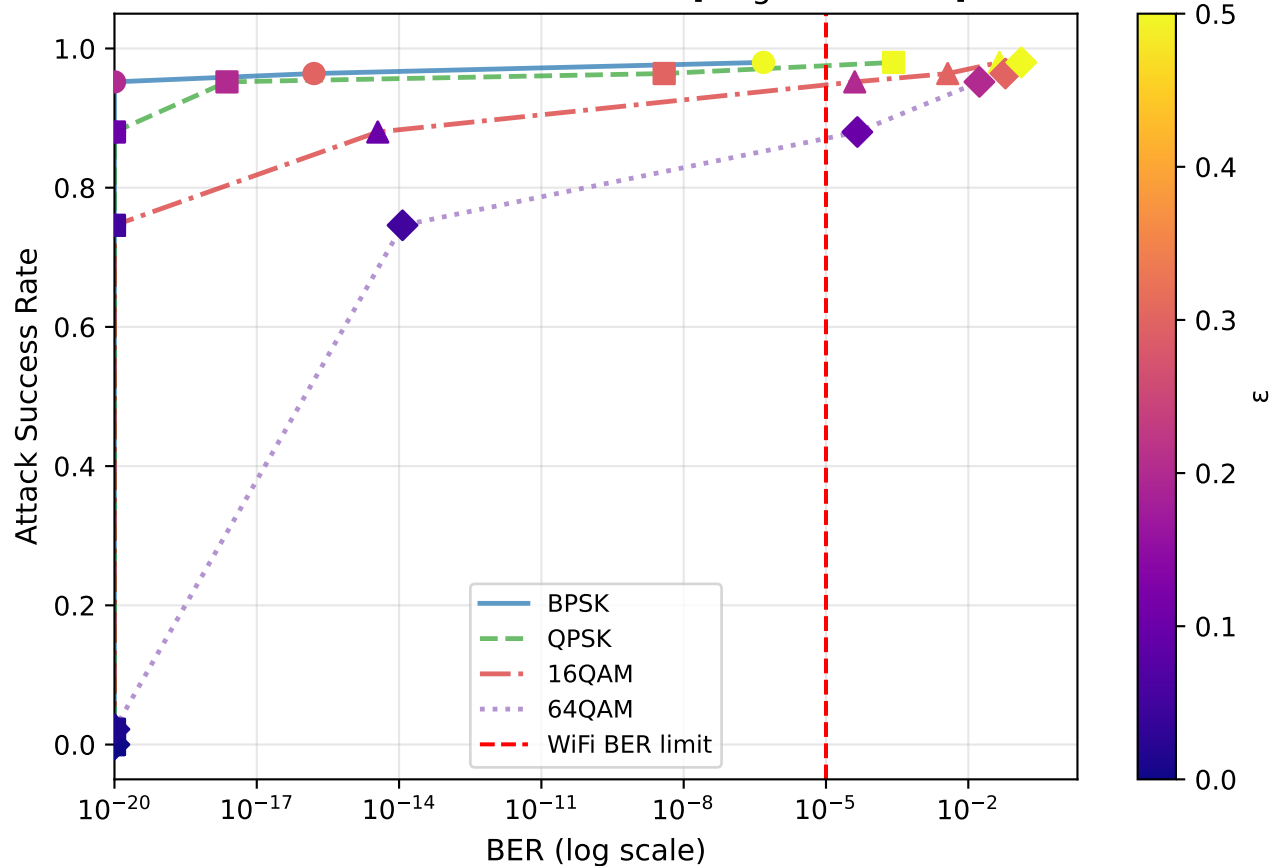
PGD — Stealthiness Tradeoff [Targeted→Dev2]
