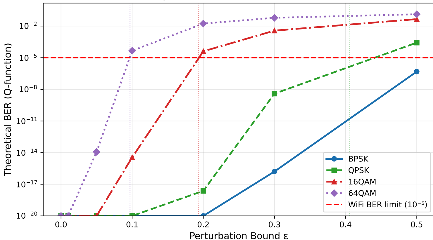
Theoretical BER vs \epsilon — 802.11 Modulations (Uniform perturbation modelled as AWGN, \sigma^2 = \epsilon^2/3 )
