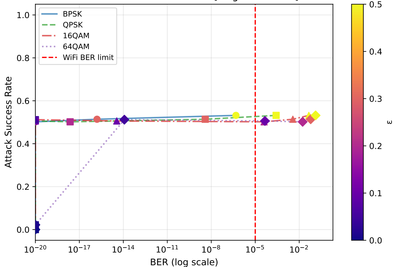
PGD — Stealthiness Tradeoff [Targeted→Dev0]
