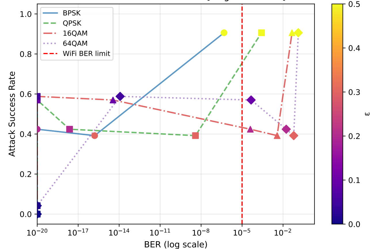
FGSM — Stealthiness Tradeoff [Targeted→Dev0]
