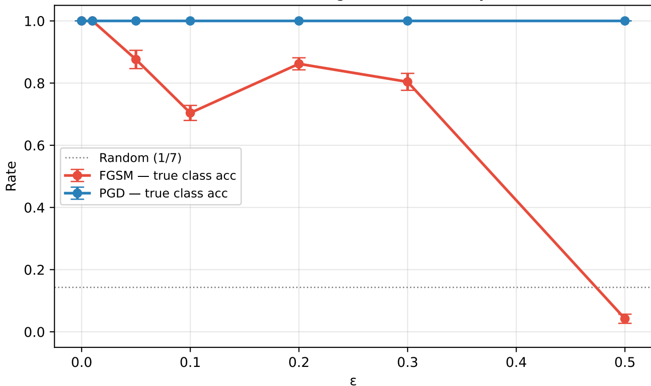
SARP IQ2CH [Untargeted] — Accuracy vs \epsilon
