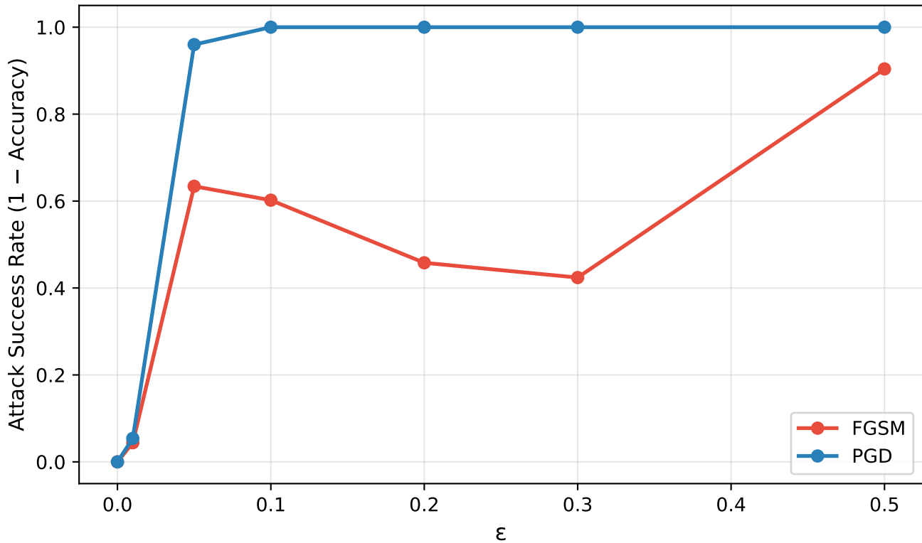
SARP [Untargeted] — Attack Success vs \epsilon
