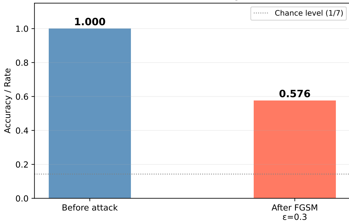
FGSM — Class 4 [Untargeted]
