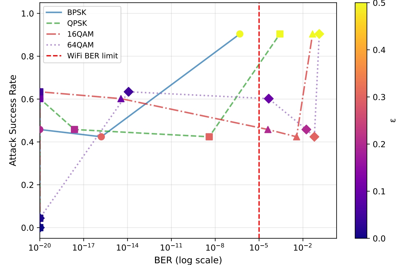
FGSM — Stealthiness Tradeoff [Untargeted]
