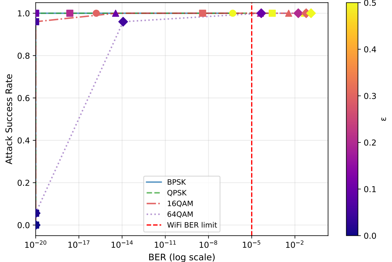
PGD — Stealthiness Tradeoff [Untargeted]
