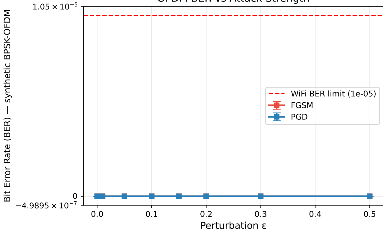
OFDM BER vs Attack Strength
