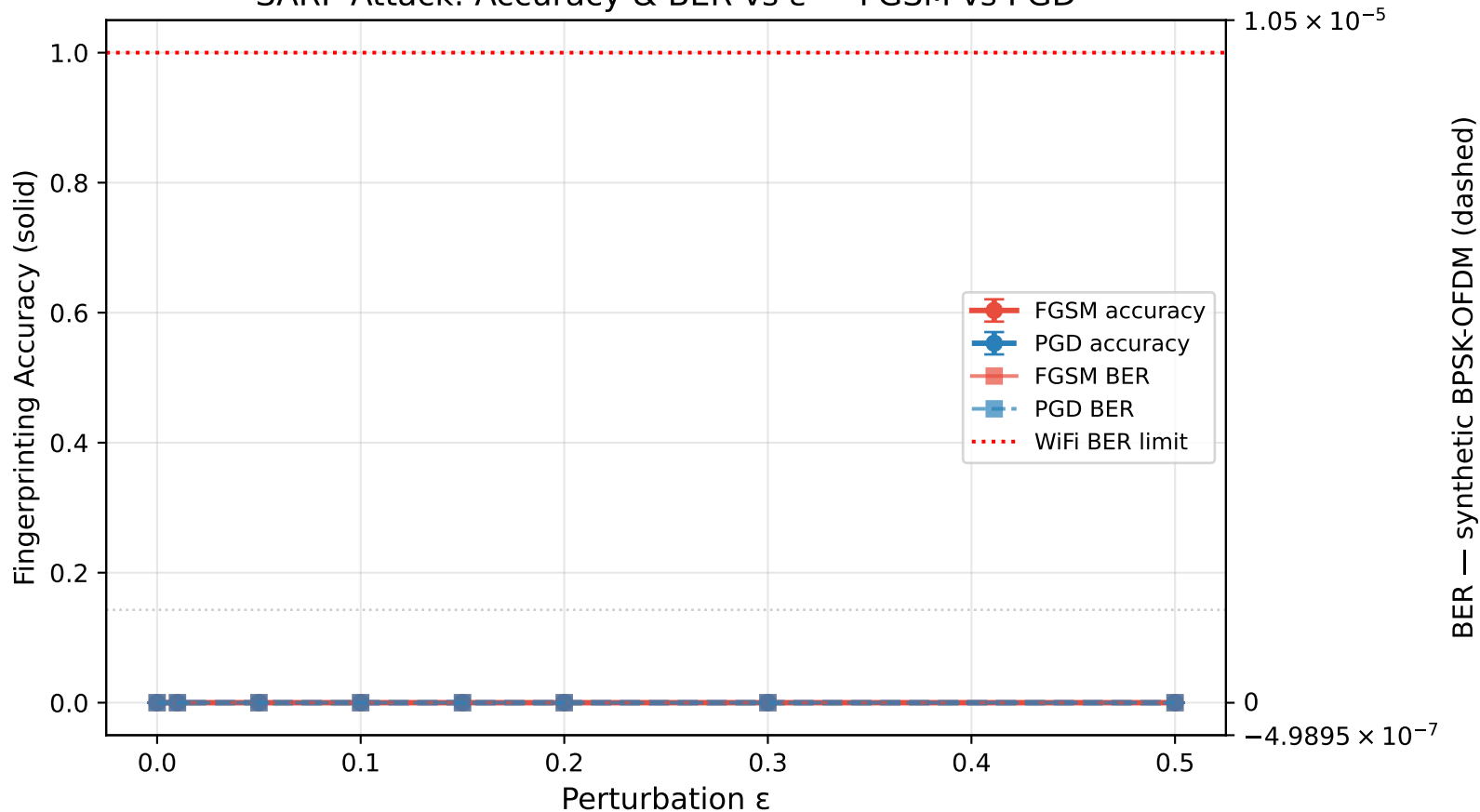
SARP Attack: Accuracy & BER vs \epsilon — FGSM vs PGD
